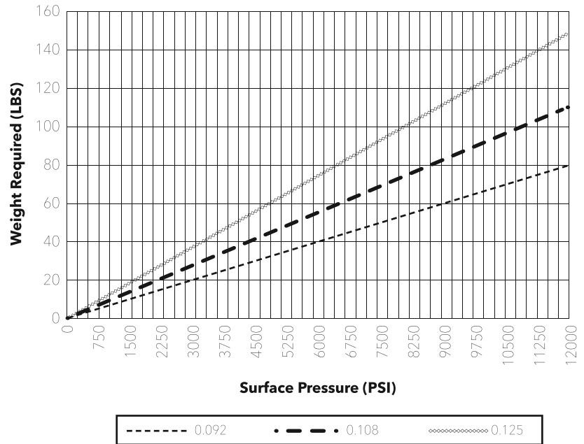
STEM WEIGHT VS WELL PRESSURE
